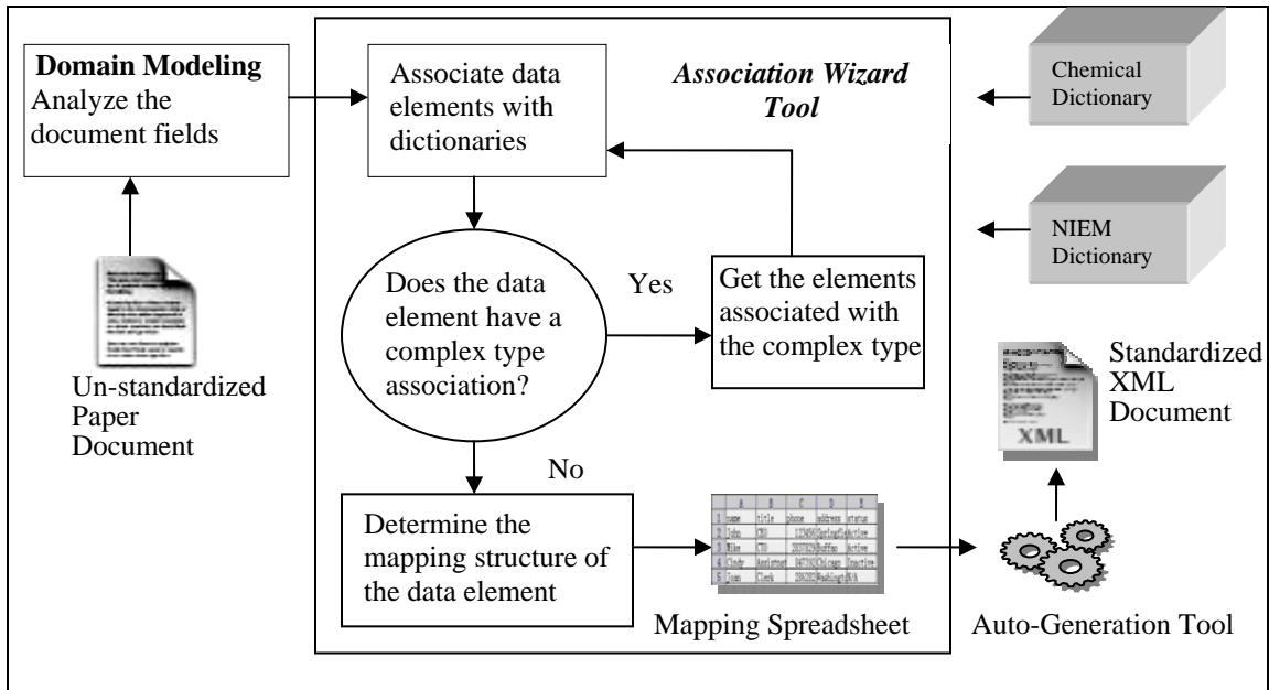
Figure 7a. Process Flow of the Association Wizard Tool
